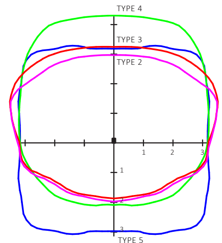
Sample Distribution Performance AR13 15M 0.2 Isofootcandle Curves Axes: X times Mounting Height
